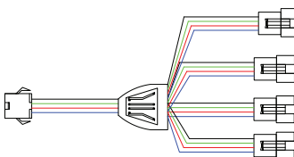
LC104 - JST 4-Way Splitter
